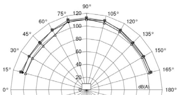
DS 10 sound pressure level horizontal diagram
