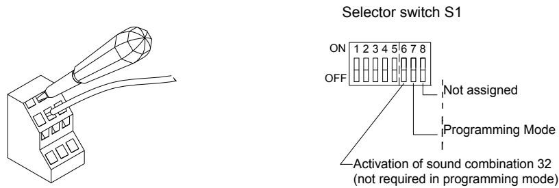
Fig. 10 Connection assignment and control elements
