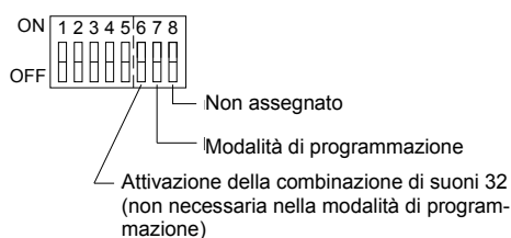
DIP switch S1
