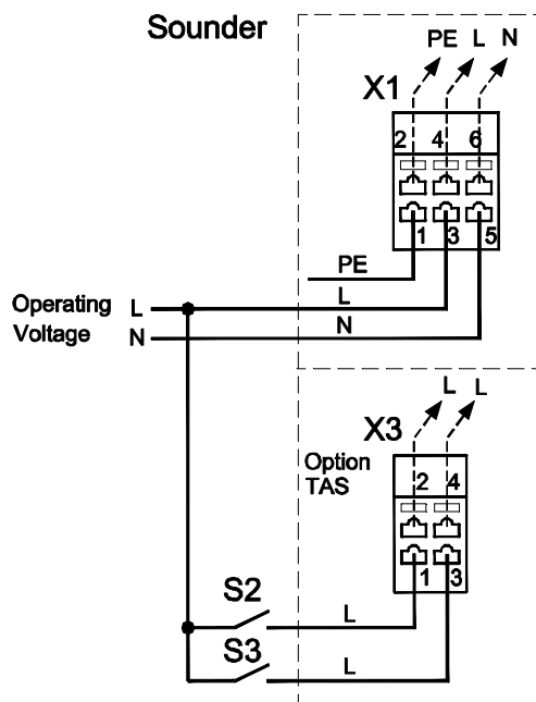
Fig. 11 Optional connection assignment TAS
