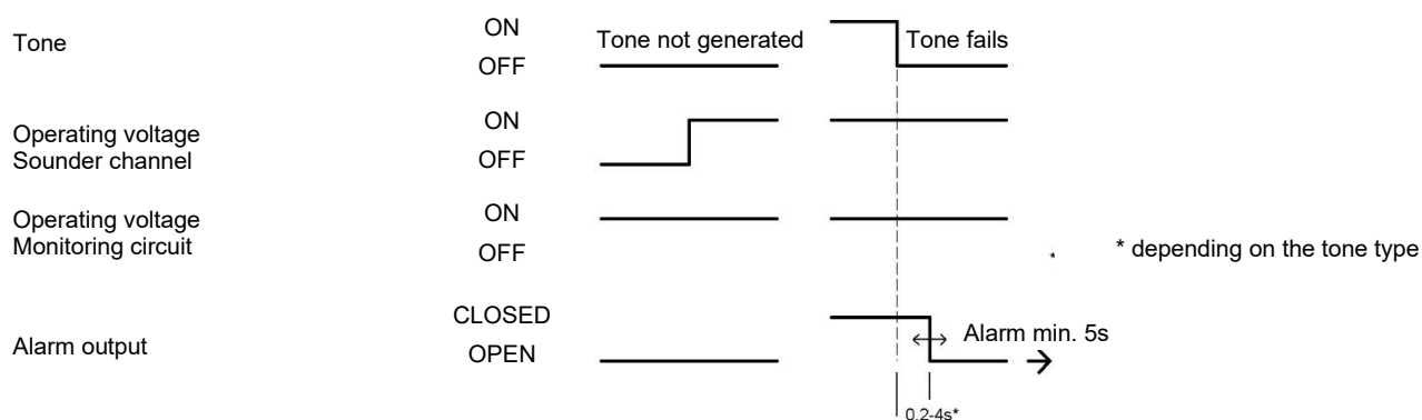
Fig. 10 Function time diagram for error
